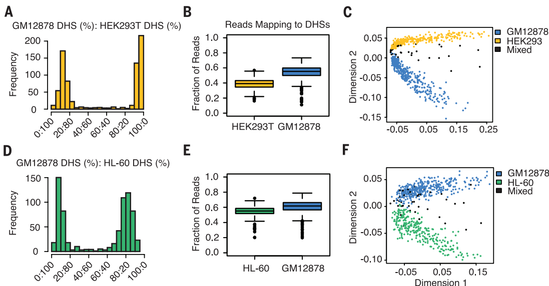
Fig. 2. Single-cell ATAC-seq deconvolutes human cell-type mixtures. (A to C) GM12878/HEK293T nuclei. (D to F) GM12878/HL-60 nuclei. [(A) and (D)] Histograms of proportions of reads mapping to cell type-specific DHSs that correspond to one cell type or the other. [(B) and (E)] Box plots of the overall fraction of reads mapping to ENCODE-defined DHSs for individual cells. [(C) and (F)] Multidimensional scaling of single-cell ATAC-seq data using pairwise Jaccard distances between cells based on DHS usage. Cell-type assignments based on proportions shown in (A) and (D).
